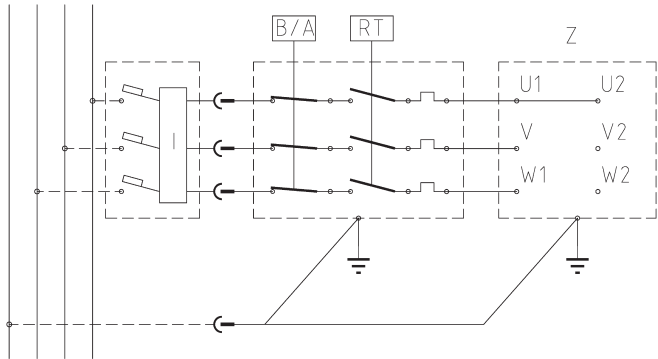
Three phase
