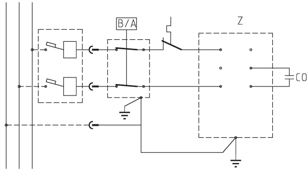
Single phase
