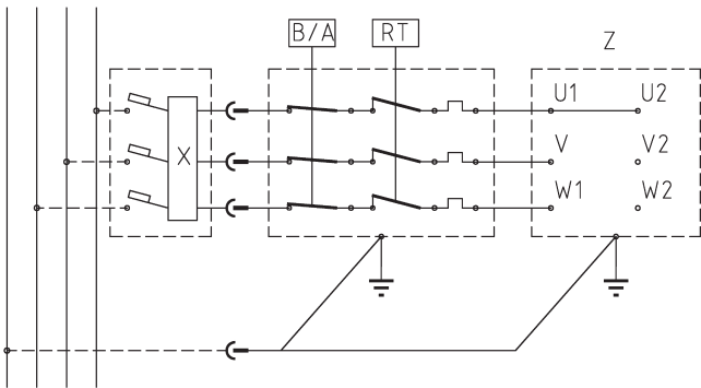
Three phase
