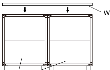
Base Cabinet
